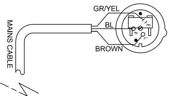
MAINS PLUG (110V)
