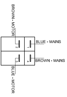
ALTERNATIVE SWITCH - 3035924
